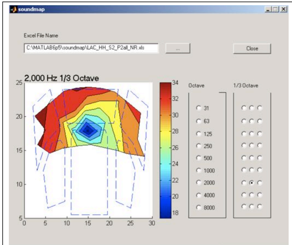
Figure 5. Contour map of Near Field Noise Reduction measurements at the Mississauga Living Arts Centre. The dashed lines indicate the location of seats and aisles on the orchestra level.
