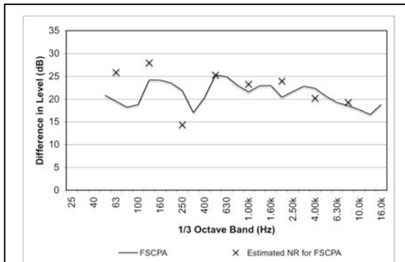
Figure 9. Calculated (X) and measured (—) Reverberant Field Noise Reduction at the Four Seasons Centre for the Performing Arts.
