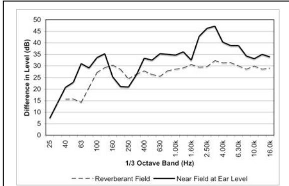
Figure 7. A comparison of Near and Reverberant Field Noise Reduction at the Mississauga Living Arts Centre.
